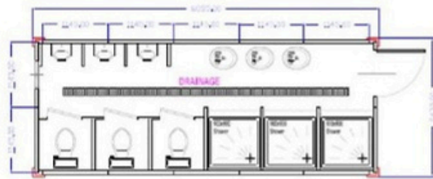
SINGLE UNIT LAYOUT (EH 114)
